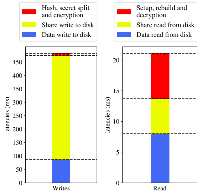
Figure 2: Breakdown of Inkpack overhead in Ceph read and write operations.
